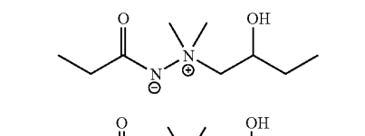
Compound G
